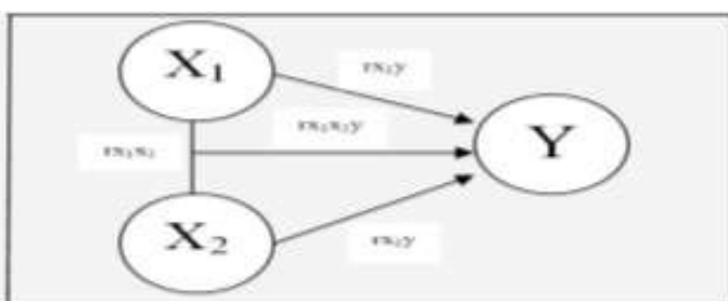
Figure 1. Multiple linear correlation models.
