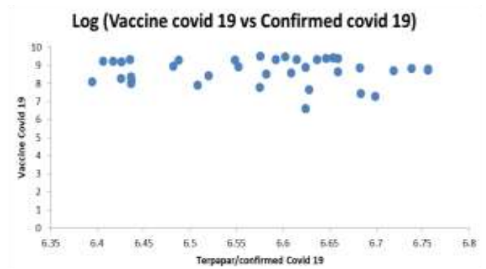
Figure 2. The corona virus 19 Confirmed plot to the COVID-19 vaccine.
