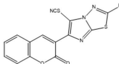
5-thiocyanato-3-(2-substituted imidazo[2,1-b]-1,3,4-thiadiazol-6-yl)-2H-chromen-2-one
