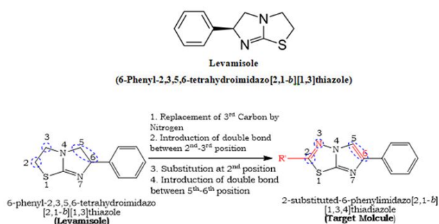
Figure 1. Synthesis of target molecule from levamisole.
