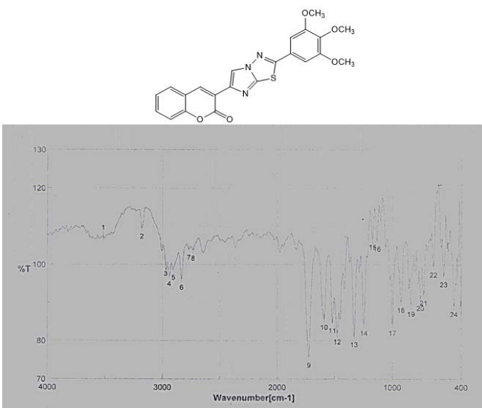
Figure 3. IR spectra of 3-(2-(3,4,5-trimethoxyphenyl)imidazo [2,1-b] [1,3,4] thiazol-6-yl)-2H-chromen-2-one. [CH 69 ].
