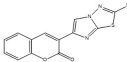
3-(2-substituted imidazo[2,1-b]-1,3,4-thiadiazol-6-yl)-2H-chromen-2-one
