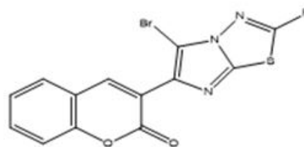
5-bromo-3-(2-substituted imidazo[2,1-b]-1,3,4-thiadiazol-6-yl)-2H-chromen-2-one:
