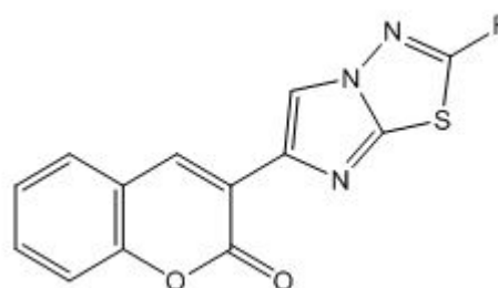
3-(2-substituted imidazo[2,1-b]-1,3,4-thiadiazol-6-yl)-2H-chromen-2-ones
