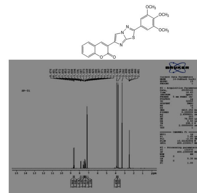
Figure 4. 1 H-NMR spectra of 3-(2-(3,4,5-trimethoxyphenyl)imidazo [2,1-b] [1,3,4] thiazol-6-yl)-2H-chromen-2-one. [CH 69 ].
