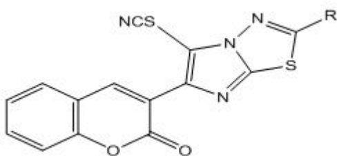
5-thiocyanato-3-(2-substituted imidazo[2,1-b]-1,3,4-thiadiazol-6-yl)-2H-chromen-2-one
