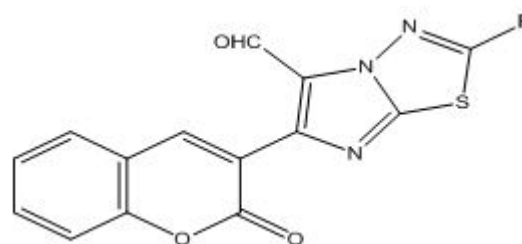
5-formyl-3-(2-substituted imidazo[2,1-b]-1,3,4-thiadiazol-6-yl)-2H-chromen-2-one
