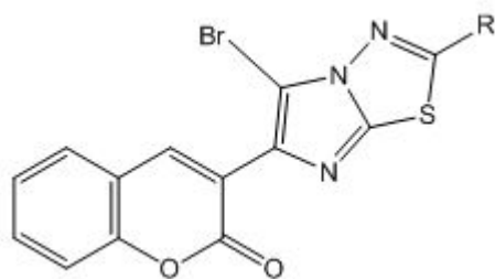
5-bromo-3-(2-substituted imidazo [2,1-b]-1,3,4-thiadiazol-6-yl)-2H-chromen-2-one
