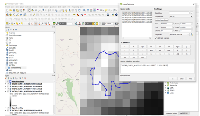
Figure 2. Raster analysis for seasonal water balance estimation of the Abay river basin.
