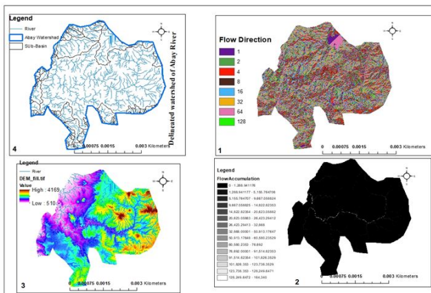
Figure 6. Water shed delineation (1. Flow Direction 2. Flow Accumulation 3. Stream flow and DEM 4. Delineated water shed and stream flow).
