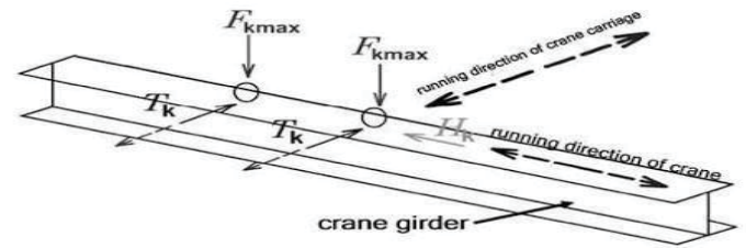
Figure 2. Loading on the crane beam.
