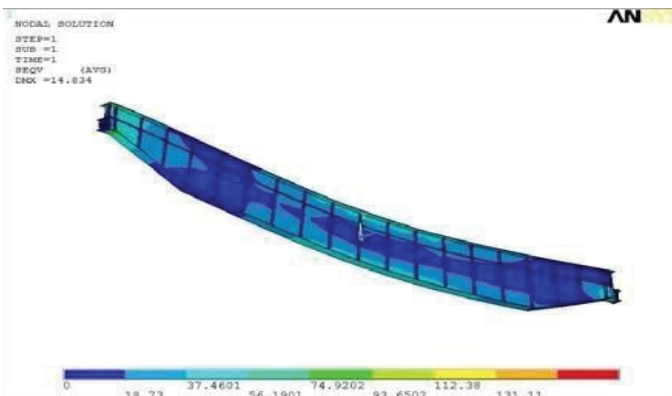
Figure 7. Von mises stress distribution of crane girder (ANSYS model).
