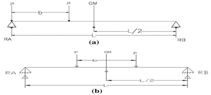
Figure 3. Worst situation of crane loading.
