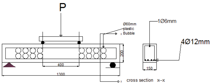
Figure 1. Illustrate the beam reinforcement and dimensions.
