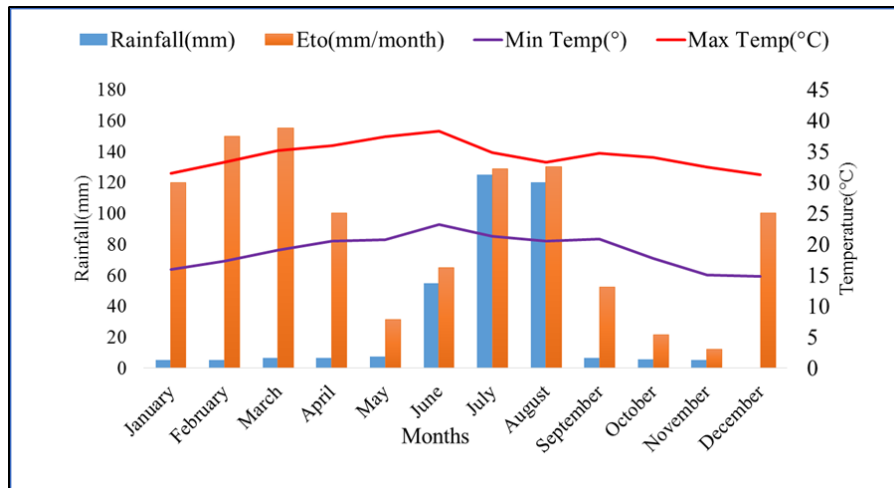
Figure 2. Climate of Study Area (1990-2019).
