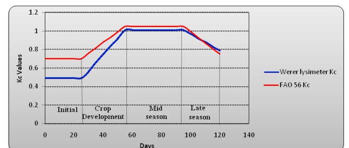
Figure 3a. Crop coefficients recommended by FAO56 for the crop (Kc FAO) and determined by lysimeter (Kc Lys) during the main cropping season.
