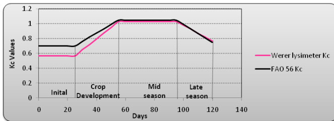
Figure 3b. Crop coefficients recommended by FAO56 for the crop (Kc FAO) and determined by lysimeter (Kc Lys) during the cool cropping season.
