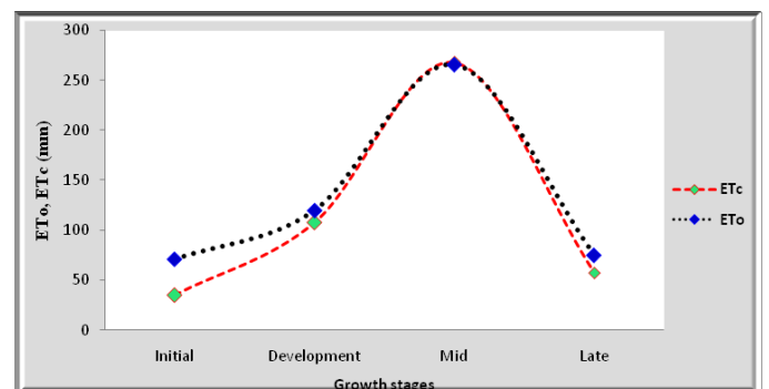
Figure 2b. Reference evapotranspiration (ETo) and crop evapotranspiration (ETC) of onion planted during the cool cropping season as a function of the growth stage.
