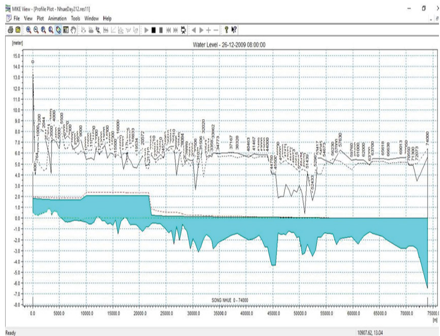
Figure 4: Hydraulic model of Nhue River basin.
