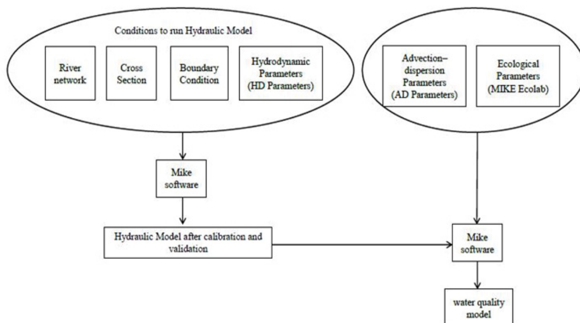
Figure 1: The principle of applying Mike 11 to calculate the changes of water quality.
