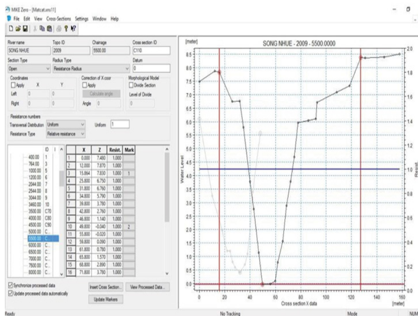
Figure 3: Cross section in Nhue River.
