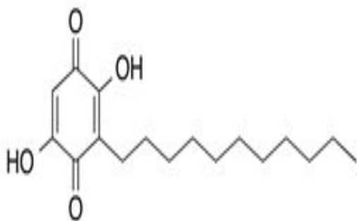
Figure 1. Chemical structure of embelin.
