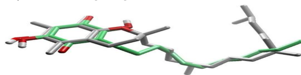
Figure 4. 3D-molecular alignment of AT (grey coloured carbon atoms) and embelin (green coloured carbon atoms) reveals similar electrostatic and steric profile. Red colour indicates oxygen atoms, while white colour indicates polar hydrogen atoms attached to oxygen atoms. Hydrogen atoms (except polar ones) are omitted for clarity.
