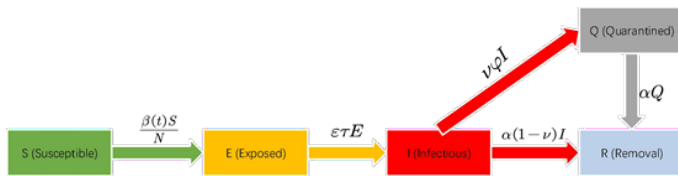
Figure 2. 2020.2.8-2020.3.30, SEIQR model, where \beta(t)=\beta(\omega E+I+Q)
