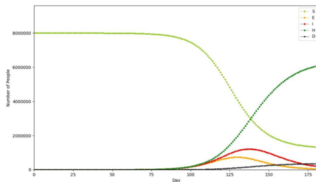
Figure 12. Result of SEIR simulation.
