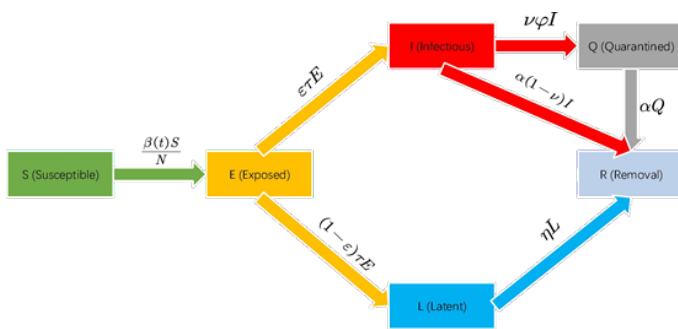
Figure 3. 2020.3.31-2020.5.16, SEIQLR model, where \beta(t)=\beta(\omega E+I+Q+\lambda L) .
