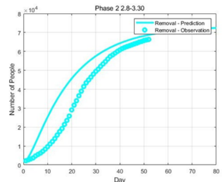
Figure 8. Result of curve fitting for the Removal R(t) in Phase 2 (2020.2.8-2020.3.30).
