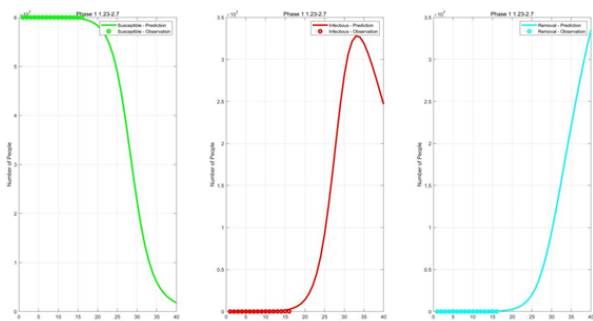
Figure 5. Result of curve fitting in Phase 1 (2020.1.23-2020.2.7).
