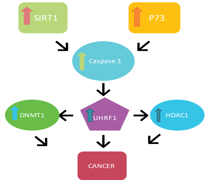
Figure 4. Upstream regulation of UHRF1: Upregulation of UHRF1 is associated with high levels of p73, SIRT1, Caspase 3, DNMT1 and HDAC1 level and ultimately leads to cancer.
