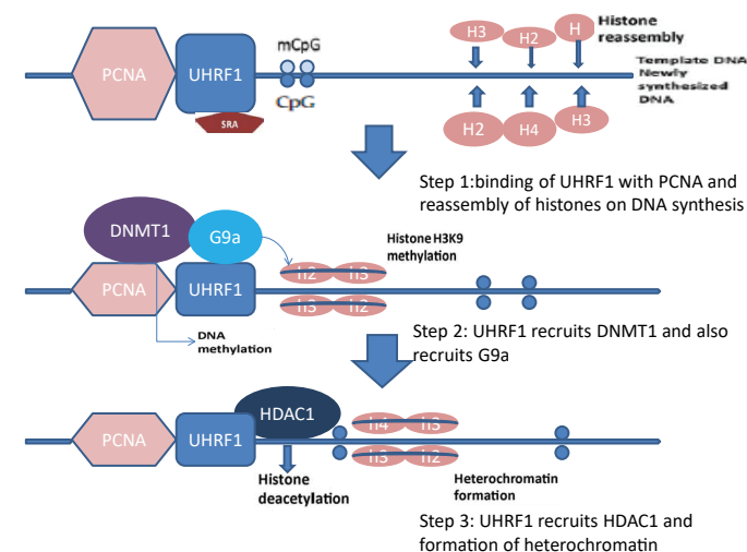
Figure 2. Mechanism of UHRF1 in heterochromatin formation. UHRF1 binds to PCNA and recognizes hemimethylated DNA through its SRA domain. UHRF1 recruits the G9a, DNMT1 and HDAC1 which methylates the h3k9 and binds with PHD domain, both DNA strands and transfer the methylation status from mother to daughter DNA strand and deacetylates the histone proteins respectively which leads to heterochromatin formation.
