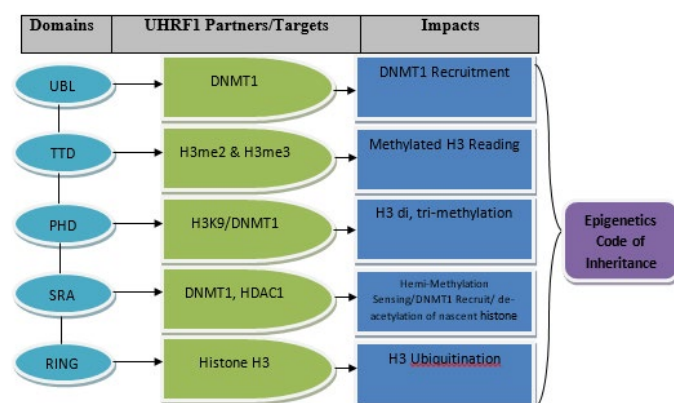
Figure 1. Construction of UHRF1: UBL (Ubiquitin-Like Domain), TTD (Cryptic Tandem Tudor Domain), PHD (Plant Homeodomain), SRA (Set and Ring Associated) and RING (Really Interesting New Gene) domains interact with DNMT1, HDAC1, H3K9 and Histone H3 proteins that lead to epigenetics code of inheritance.
