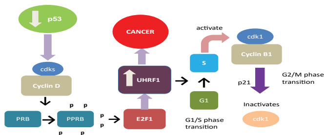
Figure 6. Role of UHRF1 in cancer.
