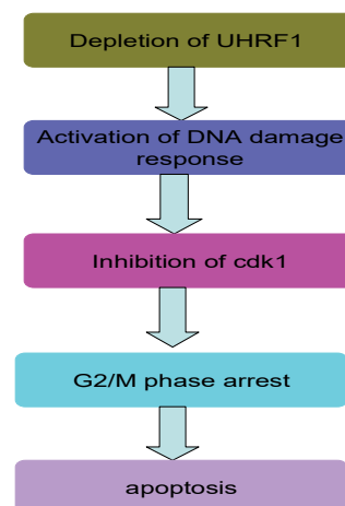
Figure 5. Depletion of UHRF1: Down-regulation of UHRF1 causes DNA damage by breaking DNA strands, cell cycle arrest in the G2/M stage by inhibiting CDK-1 and apoptosis by activating Caspase 8.
