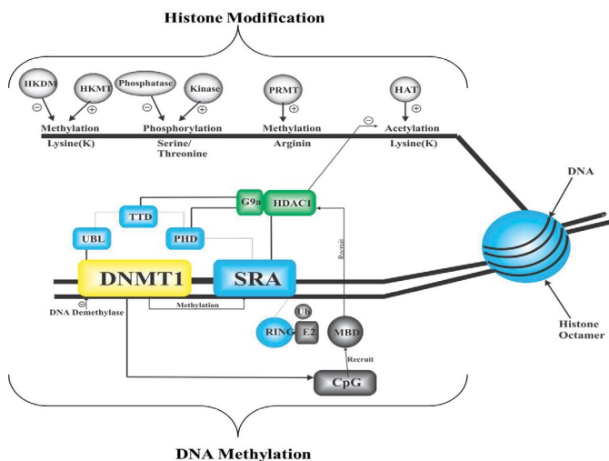
Figure 7. DNA methylation pattern in UHRF1: UHRF1 moves along DNA strands, recognizes hemimethylated CpG region and dictates DNMT1 to catalyze methylation at the target site. DNA methylation behaves as a signal for the recruitment of CpG region MBD which further recruits HDAC1 and form many genes silencing complexes.
