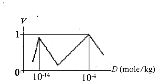
Figure 4: The type of dependence of the content of protein p53 with mice of F1 line as a function of dose D of the injected antioxidant phenosan
