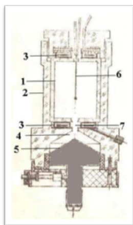
Figure 1: The construction of ampule for producing the antitumorigenic medicine with the uniform distribution of the drops of cytostatic.
