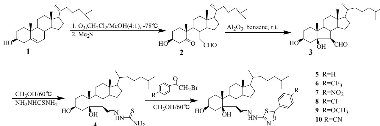
Scheme 1: Synthesis of compounds 5-10.
