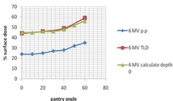
Figure 2: Comparison between the measured percentage surface dose by (TLD and P.P) and calculated by TPS with different gantry angles for 6 MV at the surface.
