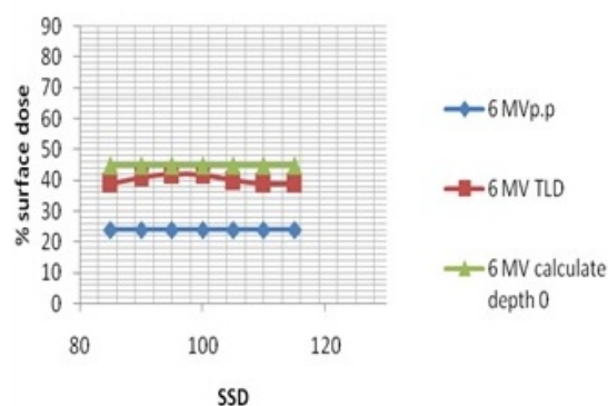
Figure 4: comparison between the measured surface dose by TLD and p. p and calculated surface dose by TPS with different SSD for 6 MV.
