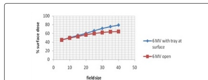
Figure 9: Comparison between open fields and the fields with tray at different field size for 6 MV.
