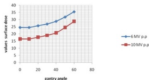
Figure 3: Absolute values of surface dose of (100 cGy /100 MU) for 6 and 10 MV.
