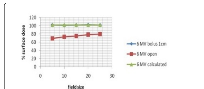
Figure 8: Comparison between the measured percentage surface dose with and without 1 cm bolus measured for different field size for 6 MV.
