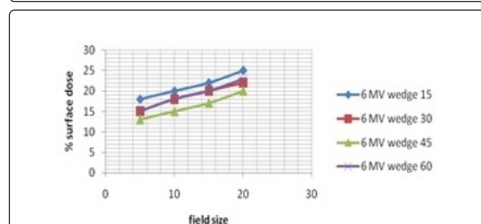
Figure 7: Comparison between the measured surface dose for wedges (15, 30, 45, 60) with different field sizes for 6 MV.
