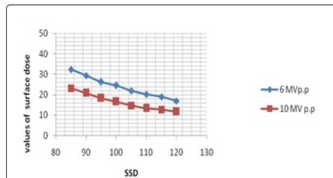
Figure 5: The measured values of surface dose by parallel plate ion chamber with different SSD for 6 MV and 10 MV at the surface.
