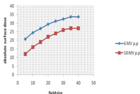
Figure 1: Absolute surface dose measured by (P.P) with different field sizes for 6 and 10 MV and SSD at surface.
