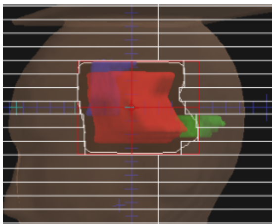
Figure 10: Beam shape with MLC in brain case for 3DCRT.
