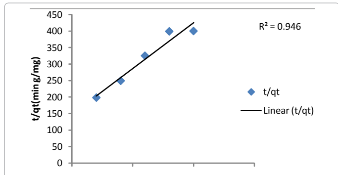
Figure 9: Pseudo - second order plot.
