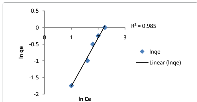
Figure 7: Freundlich equilibrium isotherm model for dye removal.
