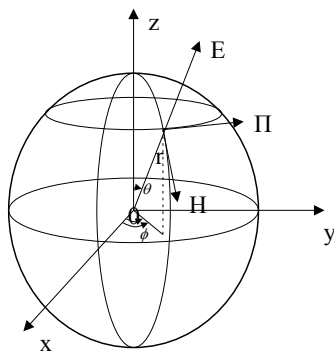
Figure 1: Representing the spherical coordinates of the observation point.
