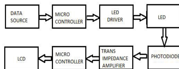
Figure 4: Building Block of the developed Li-Fi system.
