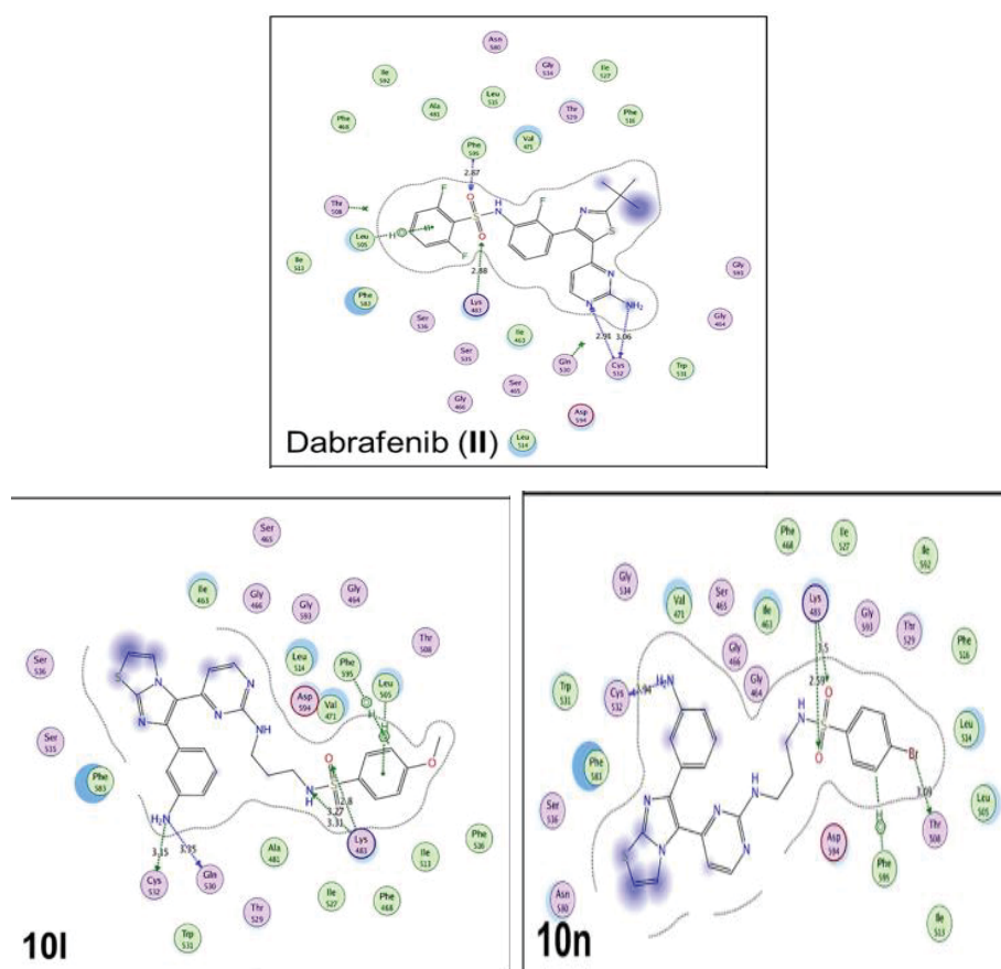
Figure 10. 2D ligand interaction of dabrafenib (II) and tested compounds (10I and 10n) with V600E B-Raf kinase domain.
