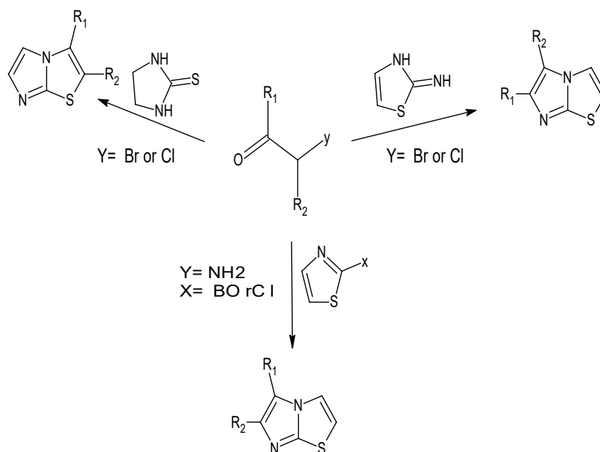
Figure 2. Methodologies to obtain imidazothiazoles from sulfur heterocycles.
