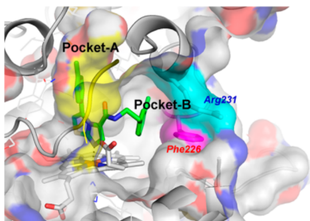
Figure 8. Crystal structure of IDO1/13b complex (green) (PDB: 4PK6). Main chain Ala260-Ser263 (yellow), Phe226 (pink), and Arg231 (cyan) are shown.
