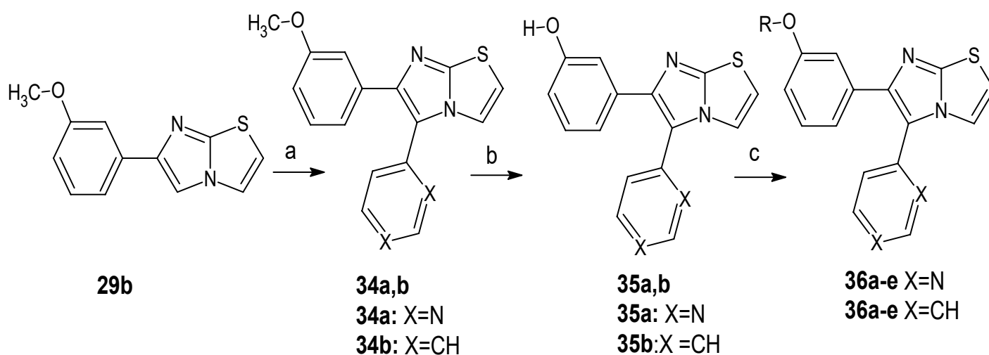
Figure 12. Reagents and reaction conditions: a) 4-Iodopyrimidine or iodobenzene, Pd(OAc) 2 , Cs 2 CO 3 , PPh 3 , DMF, 80°C, 12 h, 25-30%; b) BBr 3 , CH 2 Cl 2 , -78°C, 1 h; rt, overnight, 35-40%; c) Appropriate aralkyl halide reagent, K 2 CO 3 , anhydrous DMF, 0°C then rt, 1e2 h, 30-55%.
