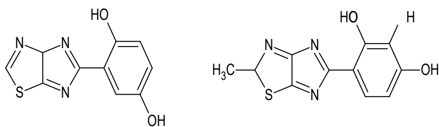
Figure 4. Imidazothiazoles endowed with polyphenolic structures.
