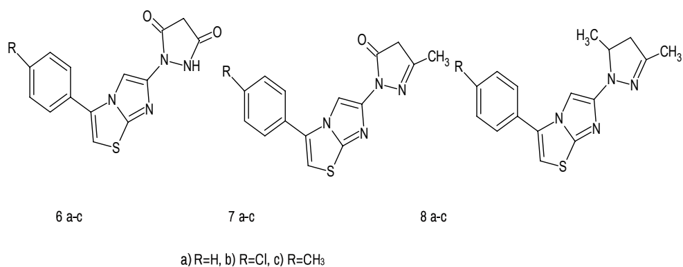
Figure 5. Imidazothiazole pyrazole derivatives.
