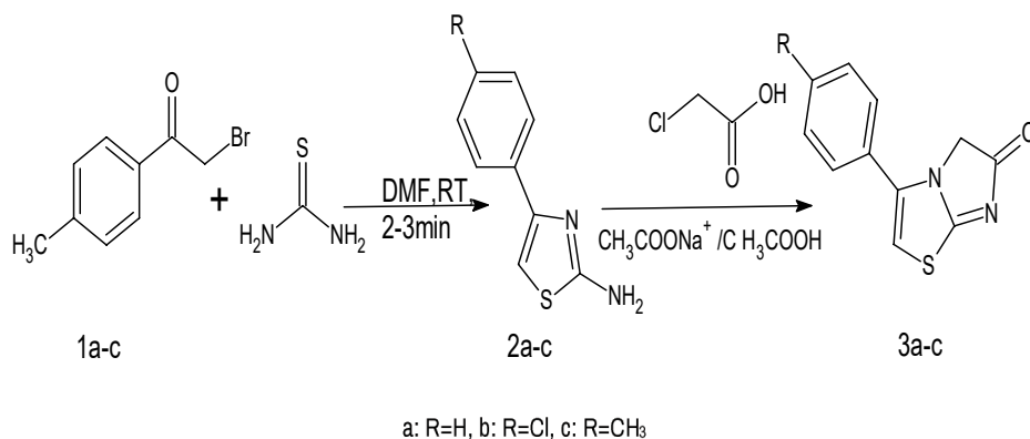
Figure 3. Synthesis of 3-arylimidazo [2,1-b] thiazol-6(5H)-one.
