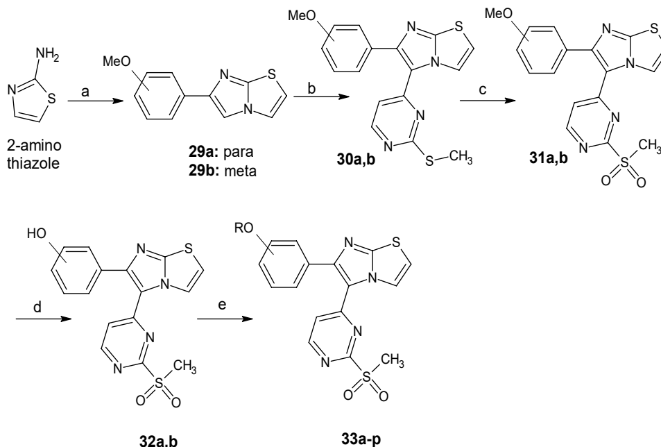
Figure 11. Reagents and reaction conditions: a) 4-Bromo-3(4-methoxyacetophenone, EtOH, reflux, 16 h, 80e85%; b) 4-Iodo-2-(methylthio)pyrimidine, Pd(OAc) 2 , Cs 2 CO 3 , PPh 3 , DMF, 80 °C, 12 h, 30e34%; c) Oxone, MeOH, H 2 O, rt, 16 h, 80e85%; d) BBr 3 , CH 2 Cl 2 , -78 °C, 1 h; rt, overnight, 55e60%; e) Appropriate substituted alkyl halide reagent or sulfamoyl chloride, K 2 CO 3 (with alkyl halide) or NaH (with sulfamoyl chloride), anhydrous DMF, 0 °C then rt, 1e2 h, 20e60%.
