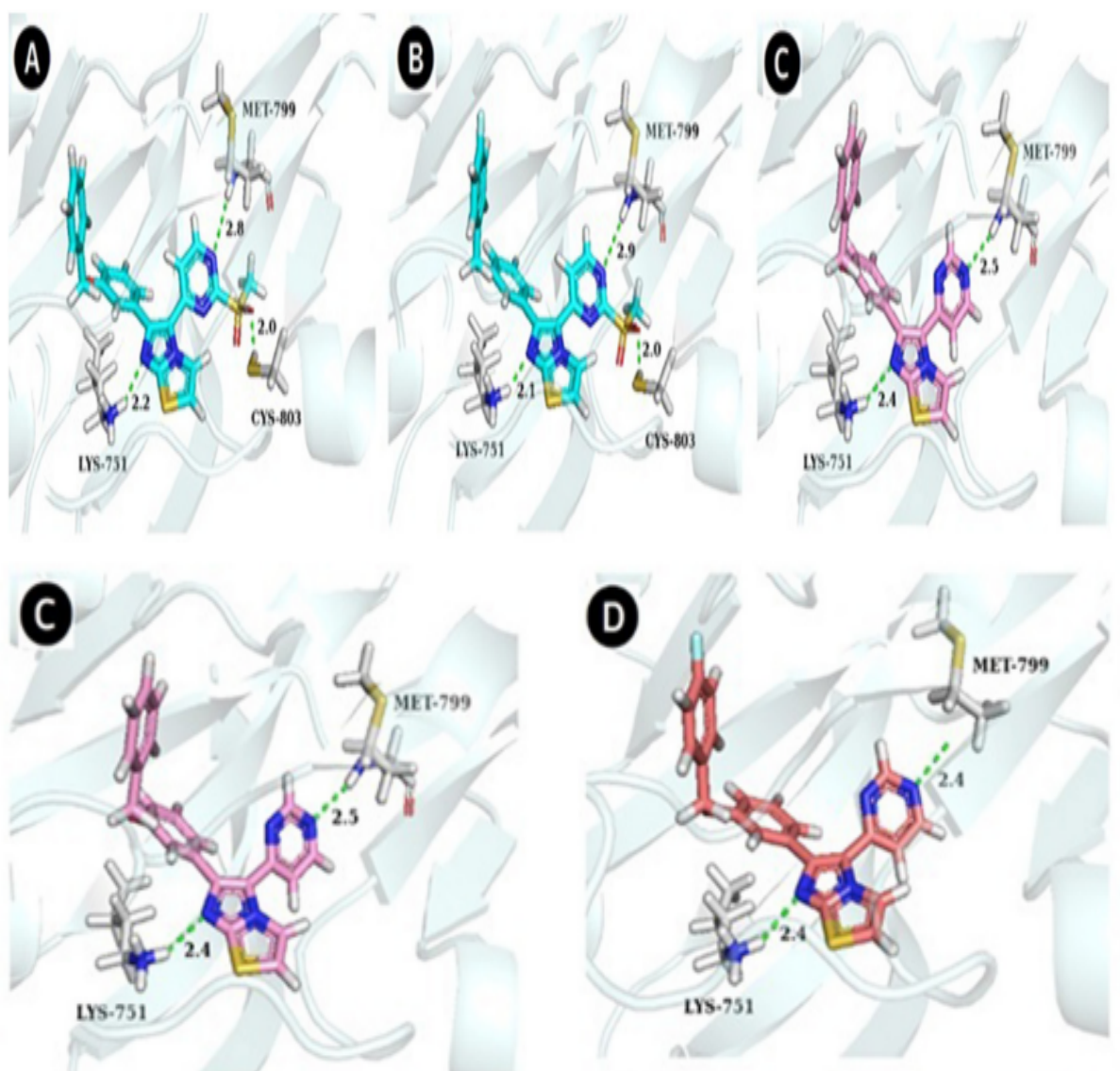
Figure 14. Best-docked poses and interactions of compounds 33k, 33l, 36a, and 36b, (respectively a-d) within the ErbB4 active site (PDB ID: 2R4B). The enzyme is represented in ribbon style. Green dashed lines represent hydrogen bond interactions while important amino acid residues are in sticks rendering.
