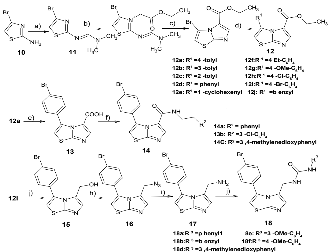
Figure 7. Synthesis of the Imidazothiazole compounds.
