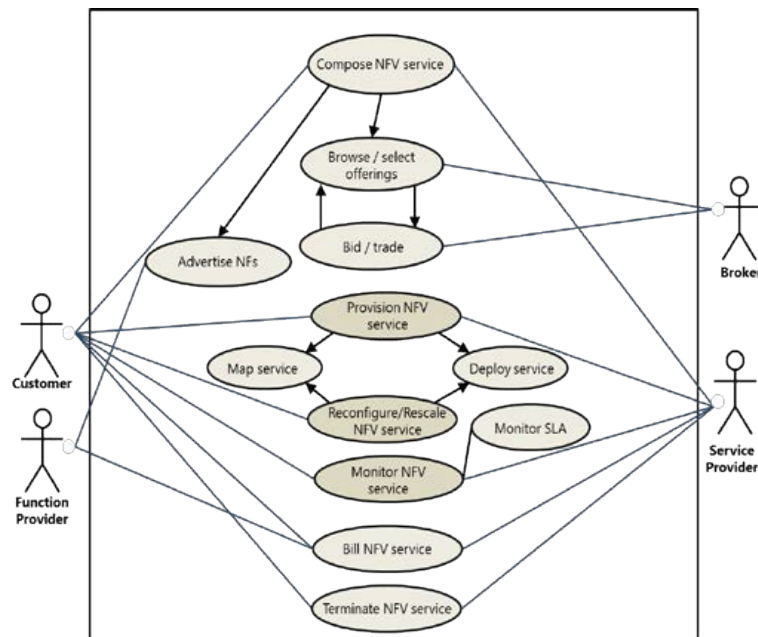
Figure 9: Overall use case diagram.
