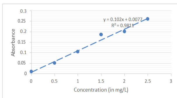
Figure 16: GRAPH 11-conc. v/s absorbance values for Zn.
