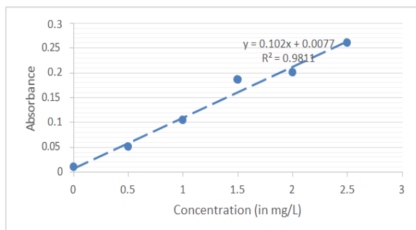
Figure 15: GRAPH 10-conc. v/s absorbance values for Ag.
