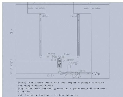
Figure 4: Hydraulic turbine.
