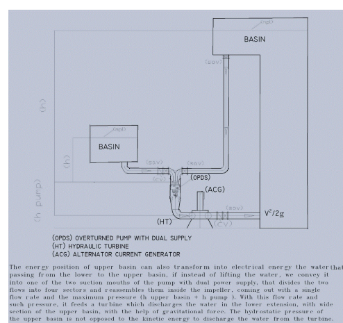
Figure 5: Overturned pump with dual supply hydraulic turbine.
