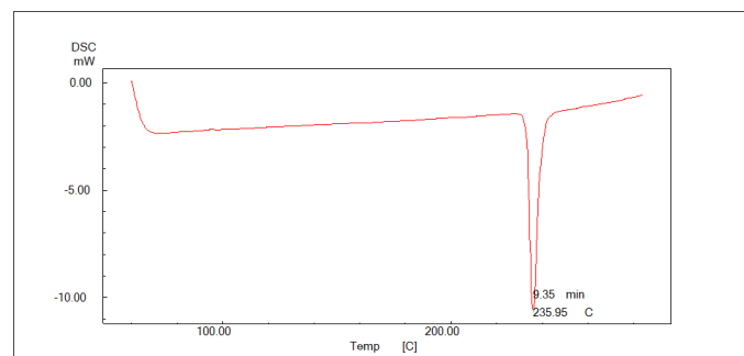
Figure 1. Differential Scanning Calorimetric (DSC) study.
