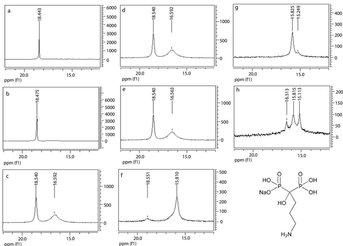
Figure 1: ^{31}\text{P} -NMR spectra of free ALN solution (700 \mu\text{l} , 100 mM) following titration with gallium nitrate (100 mM). a , free ALN; free ALN in the presence of gallium nitrate solution (100 mM), 50 \mu\text{l} ( b ), 100 \mu\text{l} ( c ), 150 \mu\text{l} ( d ), 250 \mu\text{l} ( d ), 350 \mu\text{l} ( e ), 450 \mu\text{l} ( f ), and 650 \mu\text{l} ( g ). Inset shows alendronic acid.
