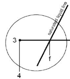
Figure 17: Condenser sub-cooling.
