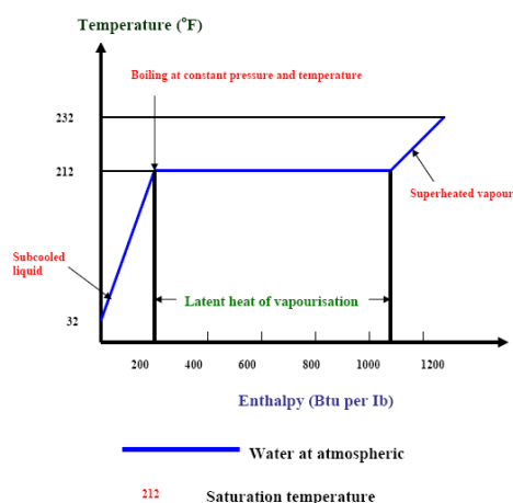
Figure 13: Water undergoing a change of state.
