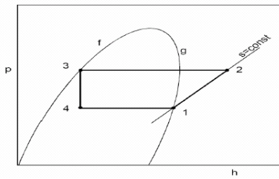
Figure 14: Refrigeration cycle.
