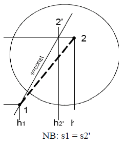
Figure 16: Isentropic compressor.
