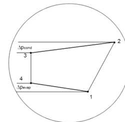
Figure 18: Pressure drops in evaporator and condenser.
