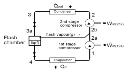
Figure 20: Liquid-suction heat exchanger cycle.
