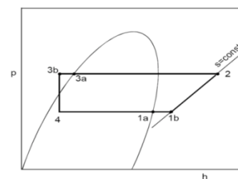
Figure 19: Diagram of liquid-suction heat exchanger.
