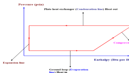
Figure 12: The ideal cycle on Pressure-Enthalpy diagram.
