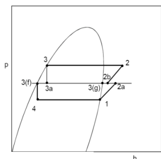
Figure 21: Cycle of multiple compressions using flash chamber.
