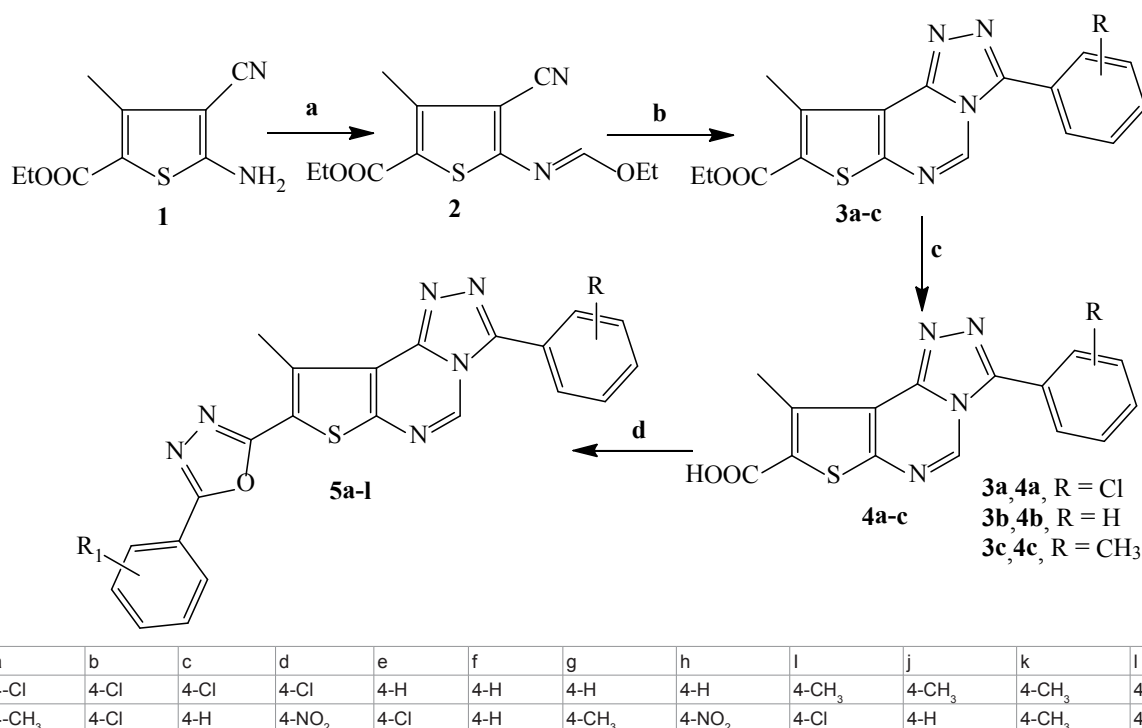
Scheme 1: Synthetic path way of preparation of 1,3,4-oxadiazole and 1,2,4-triazolethienopyrimidine derivatives.
