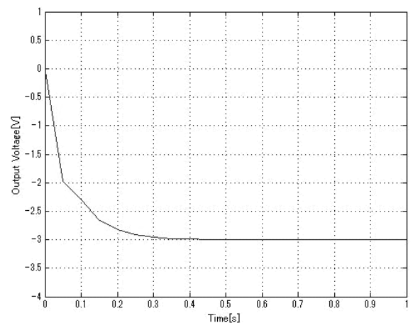
Figure 4: Output Voltage (with Compensation).
