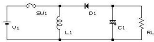
Figure 1: Schema of Buck Boost Converter.
