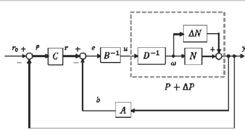
Figure 3: Nonlinear Feedback Control System.
