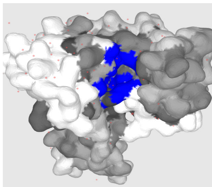
Figure 2. 3D Structure of human estrogen receptor alpha chosen binding pocket.
