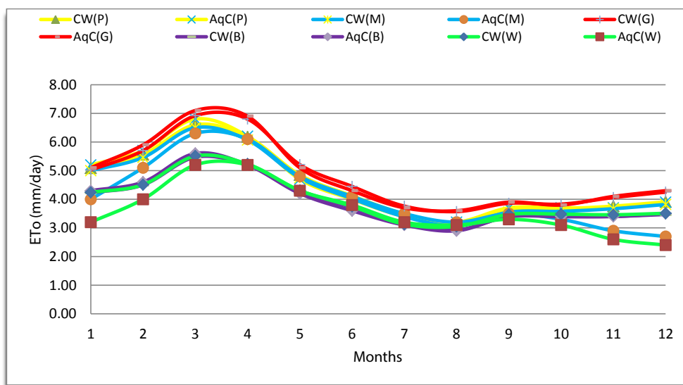
Figure 2: Long term evapotranspiration (ET o ) of the study areas (1987-2011).
