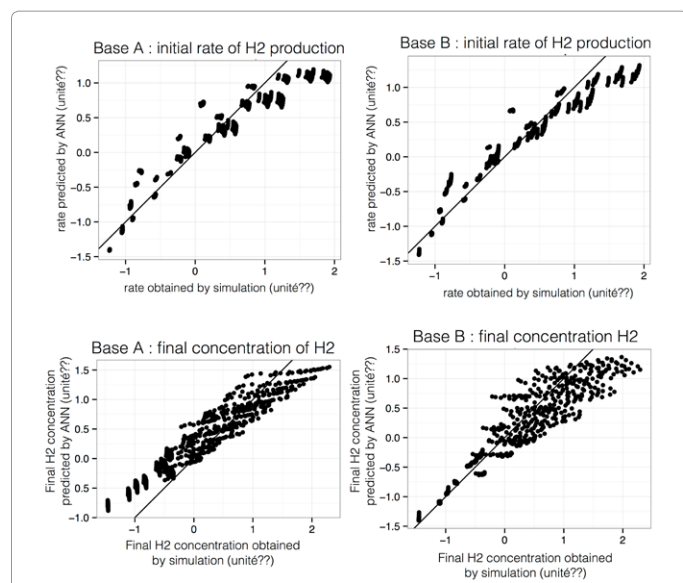
Figure 5: Performance of ANN models to predict the initial rate of production of H 2 (top) and final hydrogen concentration (bottom) for 625 data points from the validation dataset.
