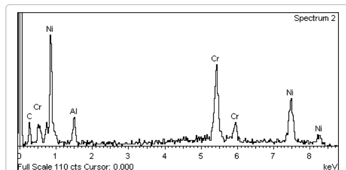
Figure 10: EDS analysis performed on the bulk sample obtained by SPS at 1200°C.
