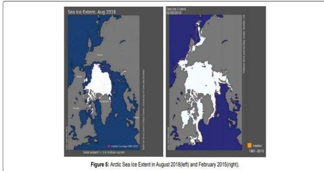
Figure 5: Arctic Sea Ice Extent in August 2018(left) and February 2015(right).
