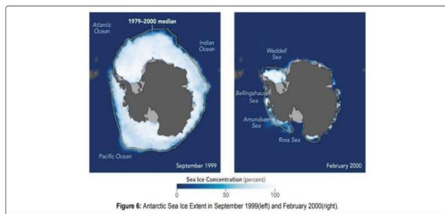
Figure 6: Antarctic Sea Ice Extent in September 1999(left) and February 2000(right).
