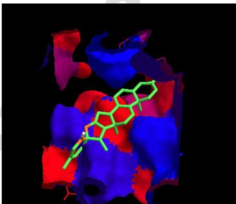
Figure 3: Docking of spirosolenol with its hydrophobic interaction.
