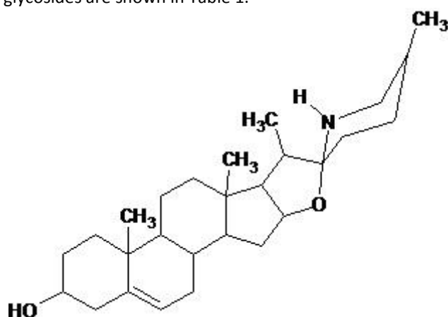
Figure 1: Structure of spirosolenol.
