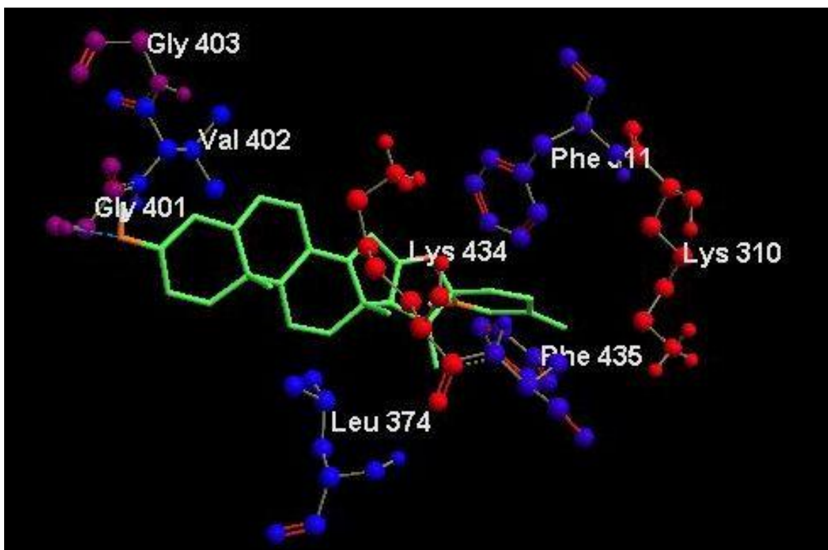
Figure 2: Docking view of spirosolenol with Human phospholipase A 2 enzyme.
