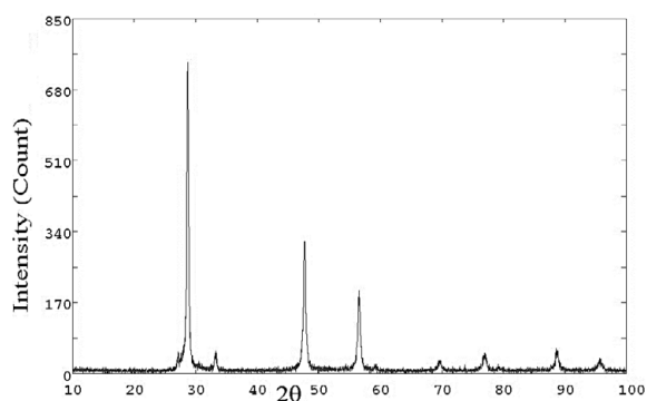
Figure 2e: XRD pattern of biofield treated ZnS sample (T4).
