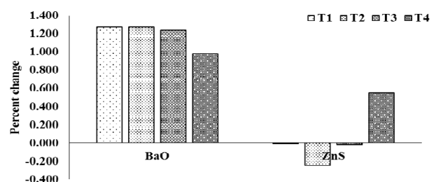
Figure 5: Percent change in density of treated BaO and ZnS as compared to control.
