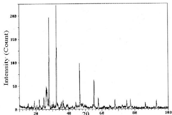
Figure 1c: XRD pattern of biofield treated BaO sample (T2).
