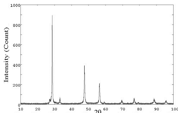
Figure 2b: XRD pattern of biofield treated ZnS sample (T1).
