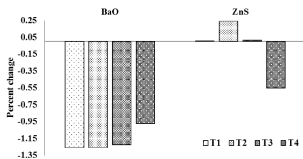
Figure 4: Percent change in unit cell volume in treated BaO and ZnS as compared to control.
