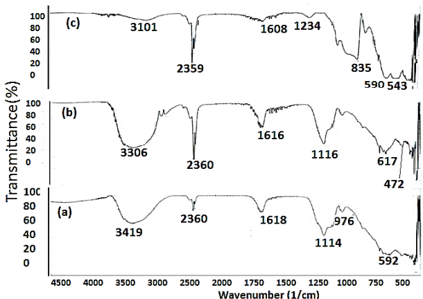
Figure 8: FT-IR spectrum of ZnS (a) Control (b) Treated T1 (c) Treated T2.
