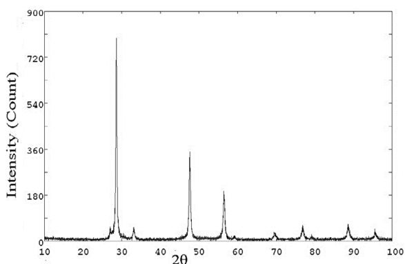
Figure 2d: XRD pattern of biofield treated ZnS sample (T3).
