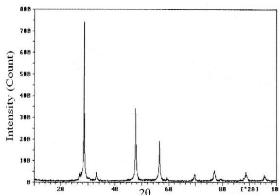
Figure 2c: XRD pattern of biofield treated ZnS sample (T2).
