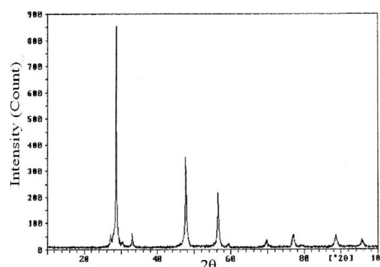
Figure 2a: XRD pattern of control ZnS sample.
