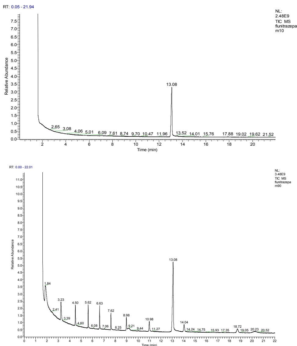
Figure 2: GC traces of flunitrazepam in the absence (upper panel) and presence (lower panel) of UV irradiations.
