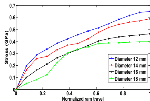
Figure 10: Stress for different punch diameters for palm oil and a fixed punch land of 4.5 mm.
