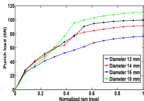
Figure 8: Punch load for different punch diameters for groundnut oil and a fixed punch land of 4.5 mm.
