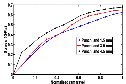
Figure 14: Stress for different punch land for palm oil and a fixed punch diameter of 12 mm.
