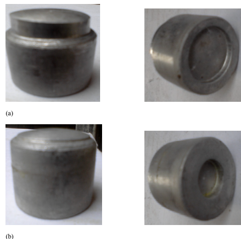
Figure 11: Extrudate rod and cup for (a) 18 mm diameter punch (b) 12 mm diameter punch.
