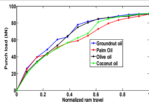
Figure 5: Punch load for different lubricants for a fixed punch diameter of 14 mm and punch land of 4.5 mm.
