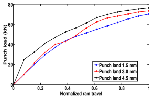
Figure 12: Punch load for different punch lands for groundnut oil and a fixed punch diameter of 12 mm.
