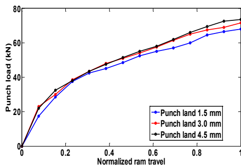
Figure 13: Punch load for different punch land for palm oil and a fixed punch diameter of 12 mm.
