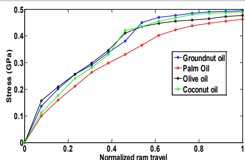
Figure 7: Stress on Al-6063 for different lubricants for a fixed punch diameter of 16 mm and punch land of 4.5 mm.
