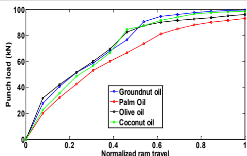
Figure 6: Punch load for different lubricants for a fixed punch diameter of 16 mm and punch land of 4.5 mm..
