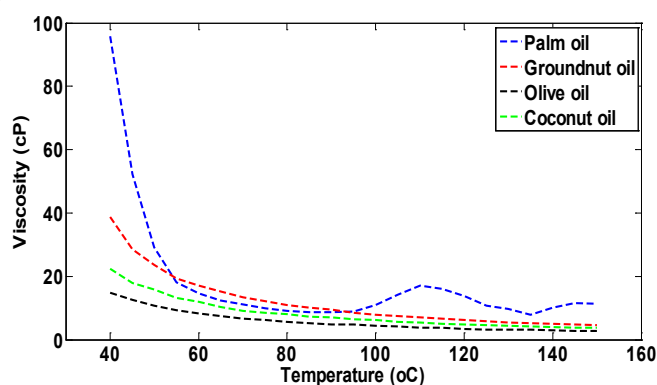
Figure 4: Viscosity of lubricants for the experiment.
