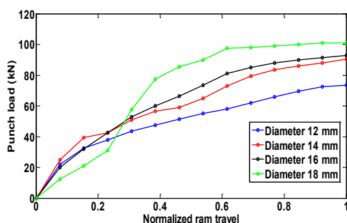
Figure 9: Punch load for different punch diameters for palm oil and a fixed punch land of 4.5 mm.
