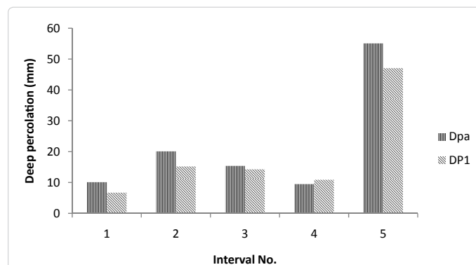
Figure 4: Comparison between observed (Dpa) and calculated (DP1) crop stage wise percolation values.
