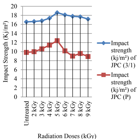
Figure 3: Impact strength of various Jute reinforced polyester composites.
