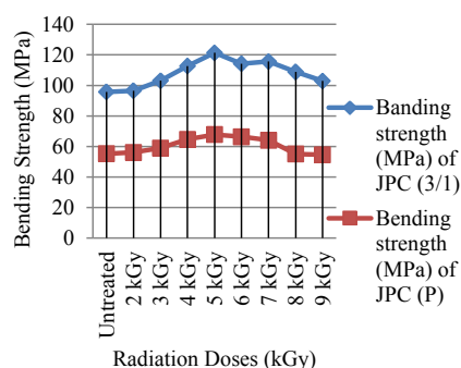
Figure 2: Bending strength of various jute reinforced polyester composites.
