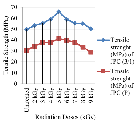
Figure 1: Tensile Strength of various jute reinforced polyester composites.
