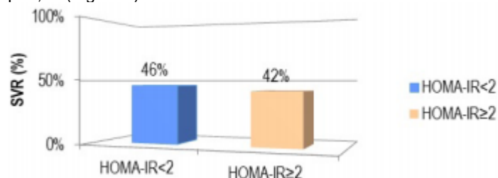
Figure 1: Efficacy of antiviral treatment in chronic hepatitis C (HCV-1) patients with HOMA-IR<2
