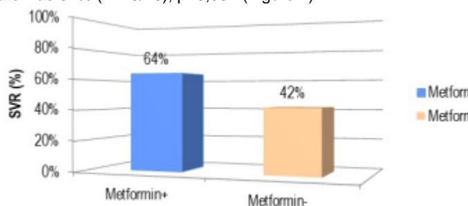
Figure 2: Efficacy of antiviral treatment in chronic hepatitis C (HCV-1) patients with HOMA-IR≥2 (with and without metformin).
