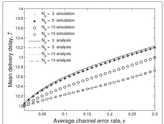
Figure 3: Mean delivery delay versus mean channel error rate \epsilon for d_0=0.6667 .
