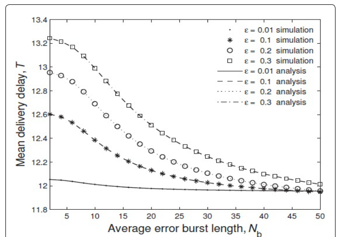
Figure 4: Mean delivery delay versus average error burst length N_b for d_0=0.6667 .
