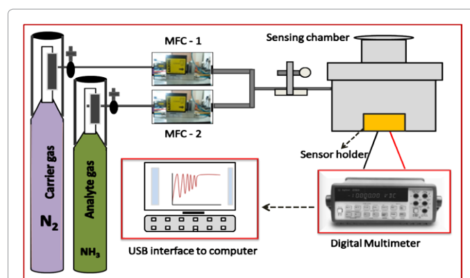
Figure 1: Schematic diagram of the experimental setup used for gas sensor performance analysis.
