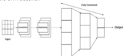
Figure 3. CNN Classifier Architecture.
