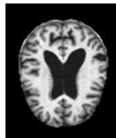
Figure 6. Pre-Processed image.
