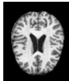
Figure 6. Pre-Processed image.
