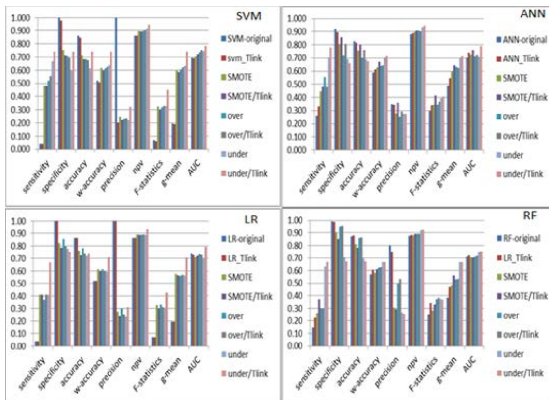
Figure 3: Performance of different ML algorithms using different sampling techniques (family data).
