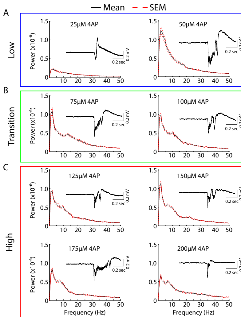
Figure 3: Concentration-dependent differences in epileptiform spectrograms. Averaged spectrograms of activity induced by different concentrations of 4AP. The mean is plotted in black solid line and standard error (SEM) in red broken line (A) Low 4AP concentrations (B) Transition concentrations (C) High concentrations. Insets are of single representative epileptiform bursts elicited by the corresponding 4AP concentration.
