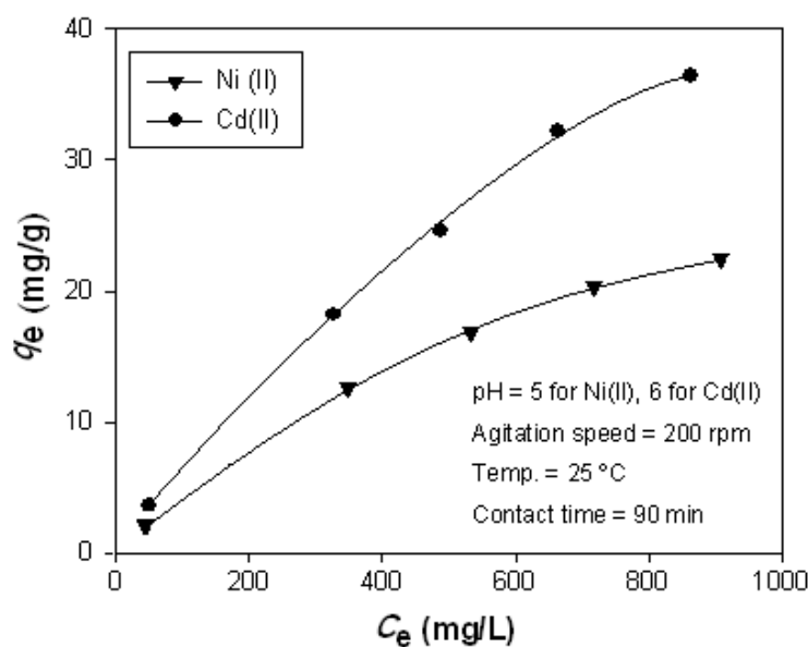
Figure 7. Effect of initial metal ion concentration on adsorption capacity.
