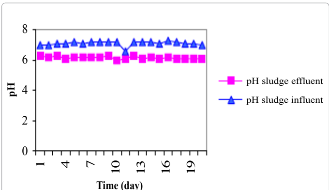
Figure 6: pH sludge before and after treatment in the digester [12].
