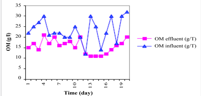
Figure 5: Organic matters before and after treatment in digester [12].
