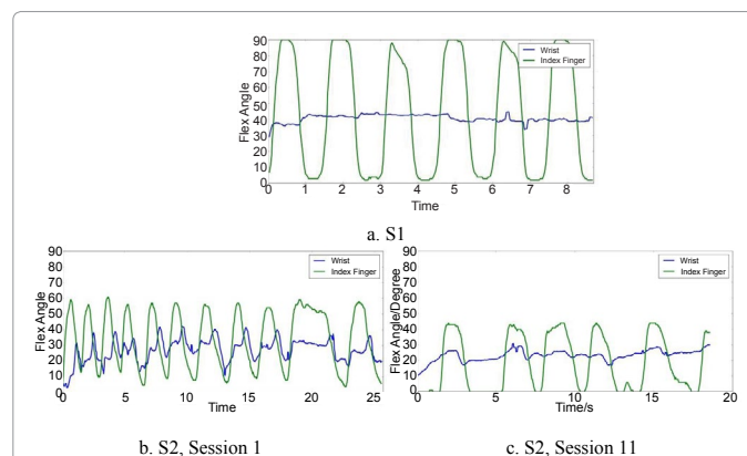
Figure 3: The flexion angle during finger flexion and extension calibration
