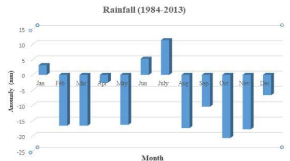
Figure 3: Monthly average anomalies.
