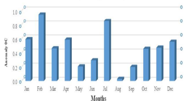
Figure 6: Average maximum temperature anomalies.
