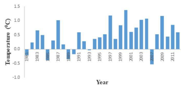
Figure 5: Annual average maximum temperature anomalies.
