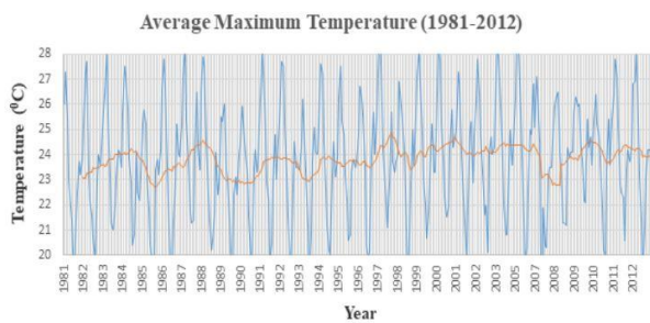
Figure 4: Average annual maximum temperature (1981-2012).
