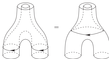
Figure 14: The compatibility condition of a bialgebra.
