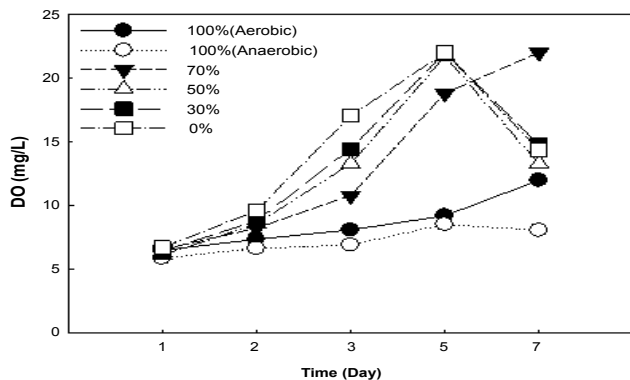
Figure 2: Dissolved Oxygen Concentration Trends at Different Shading Rates.
