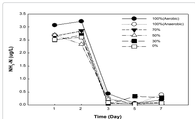
Figure 4: Ammonia Nitrogen Concentration Trends at Different Shading Rates in Water Bodies.
