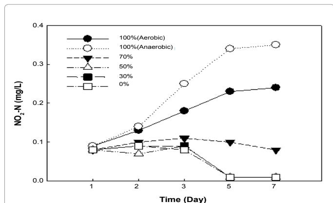
Figure 6: Nitrite Nitrogen Trends at Different Shading Rates in Water Bodies.
