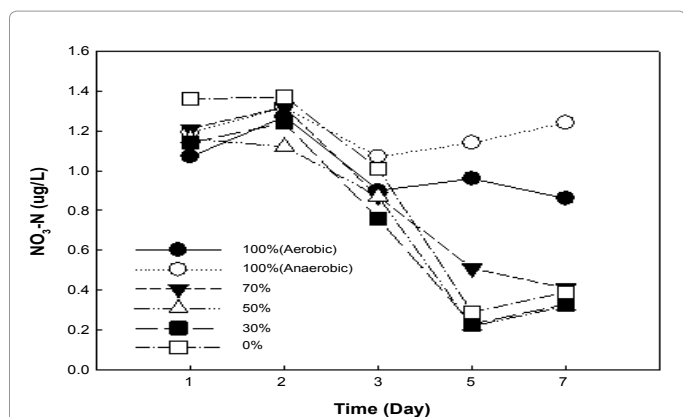
Figure 5: Nitrate Nitrogen Concentration Trends at Different Shading Rates in Water Bodies.
