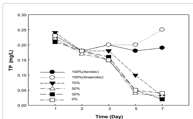
Figure 8: Total Phosphorous Content Trends at Different Shading Rates in Water Bodies.
