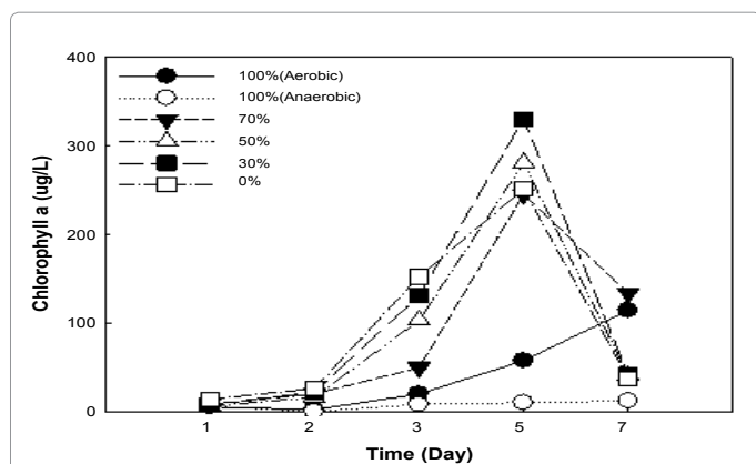
Figure 3: Algae Concentration Trends at Different Shading Rates in Water Bodies.
