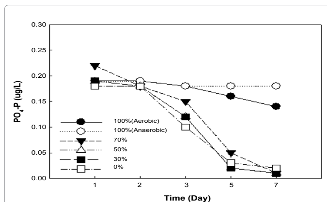
Figure 7: Orthophosphate Concentration Trends at Different Shading Rates in Water Bodies.
